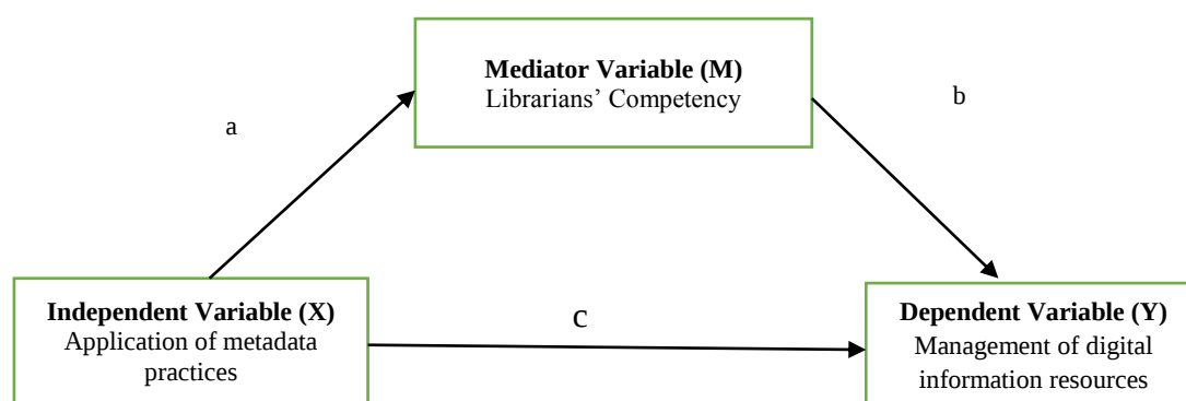
FIG 1: Mediation Analysis
