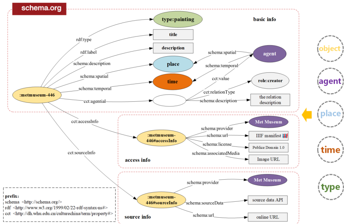
FIG. 2. The unified data model
