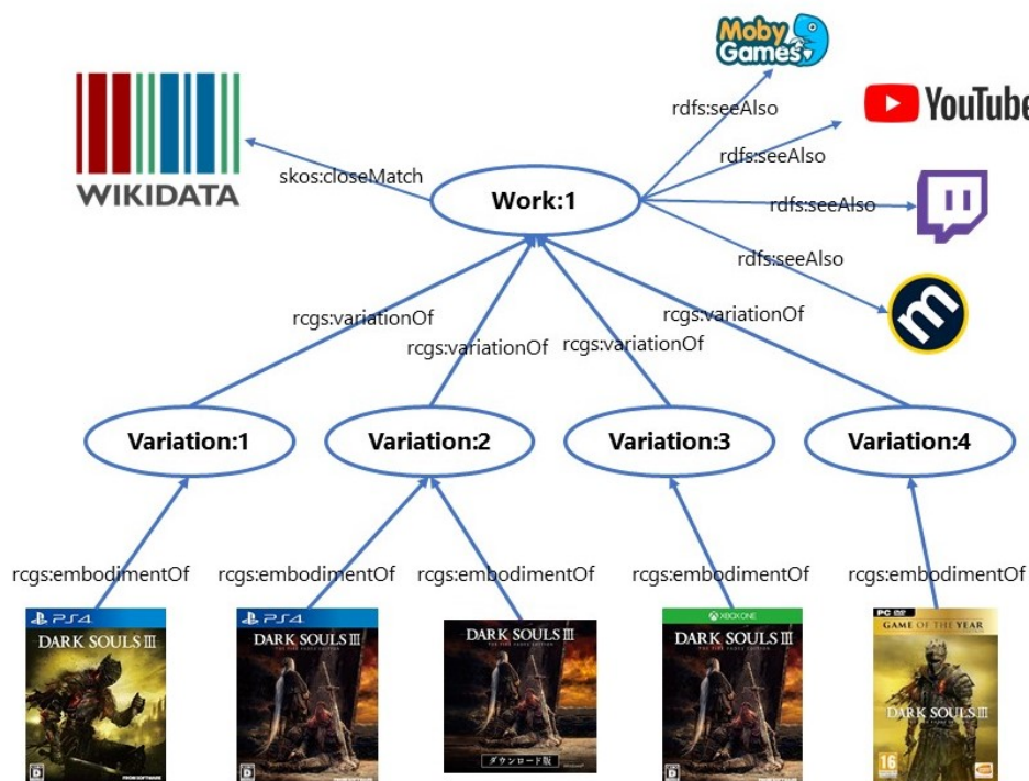
FIG. 3. Applying “DARK SOULS 3” on the metadata model
