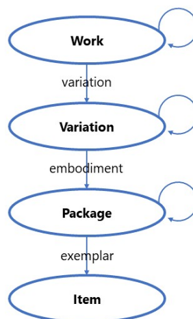
FIG. 2. Main entities of metadata model.
