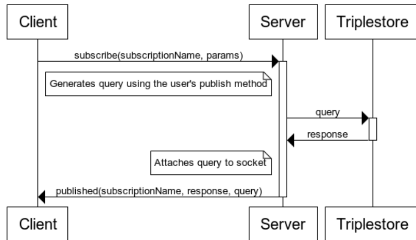
FIG. 2. Sequence for subscribing and publishing.
