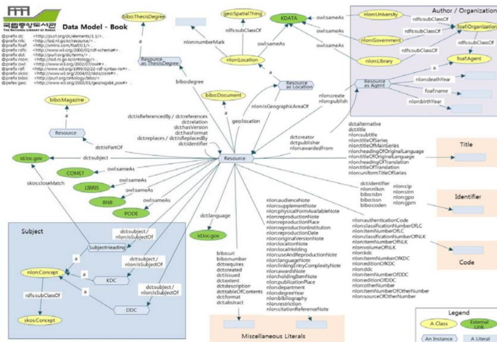
FIG. 2. NLK ontology Source: NLK Home Page
