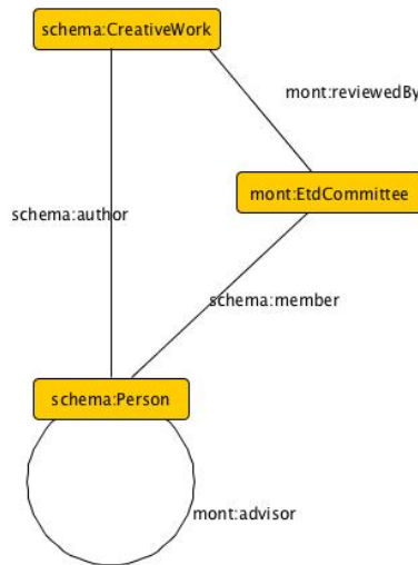
FIG 1: Relationships derived from DC records
