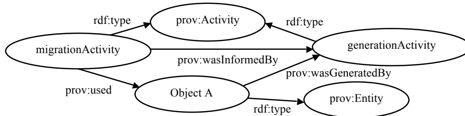
FIG.7. Relationship between Activities in PROV
