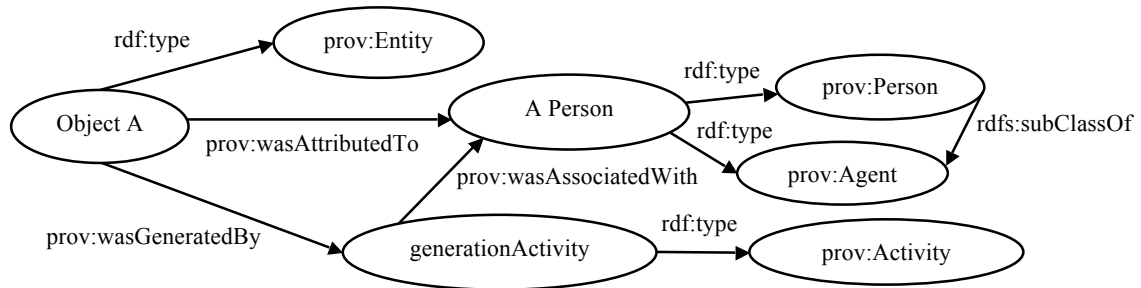
FIG.3. Provenance graph of Agent responsible for the generation of Digital Object A Using PROV
