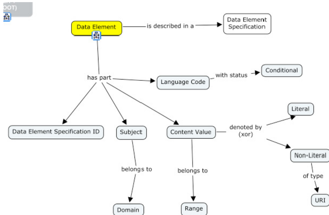
Figure 1 – Concept map for Data elements (ISO/IEC 19788, Annex C, p. 50)
