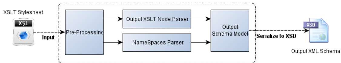
FIG. 1: Solution Architecture
