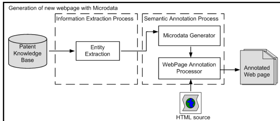
FIG.4. Overall process of generating new webpage with microdata
