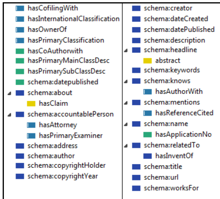
FIG.2. Overview of the Properties in Patent Ontology
