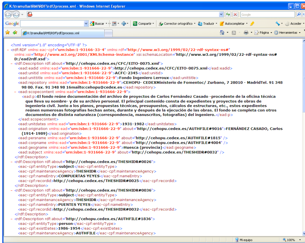
FIG. 3. Sample RDF file generated from an EAD finding aid
