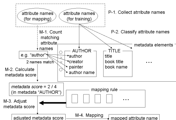
FIG. 1. Flow of metadata mapping.
