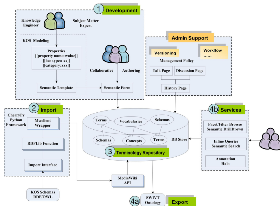
FIG. 1. Architecture of the SMW-empowered Terminology Registry
