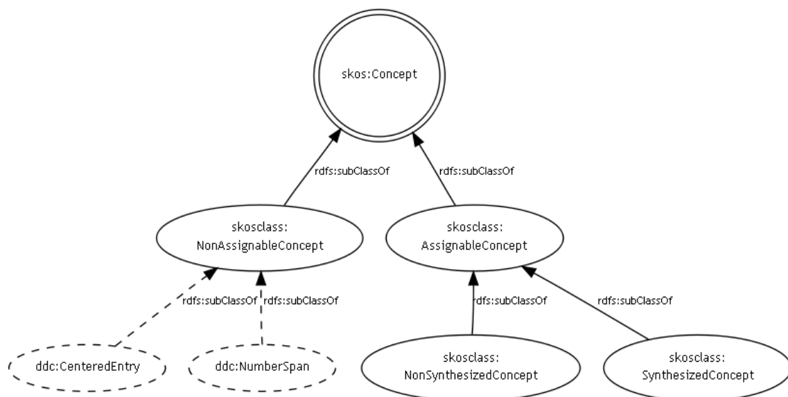
FIG. 1. Extended concept types.
