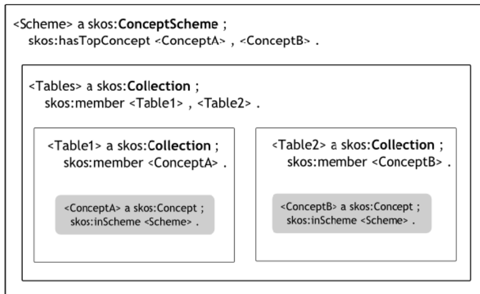
FIG. 2. Nesting of collections in combination with assertions of top concepts allows for random access to top concepts of collections.
