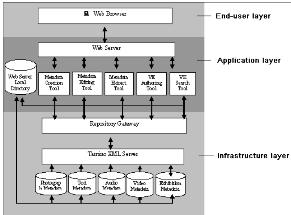
FIG. 5. Architecture of VAES.
