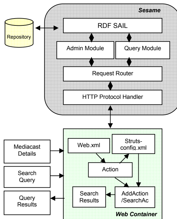
Figure 7: Publish/Subscribe architecture
