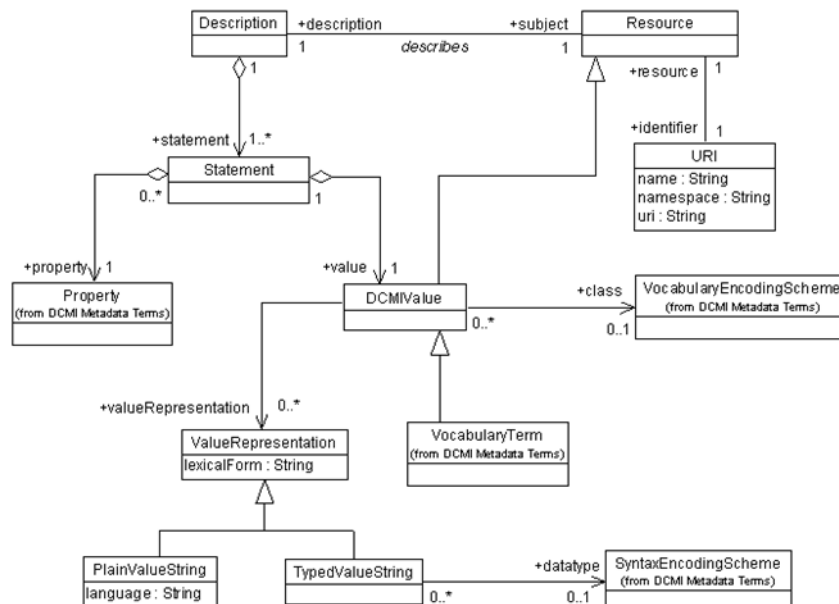
Figure 3: A DCMI Metadata Description diagram as a modified version of the DCMI description model of the DCAM.
