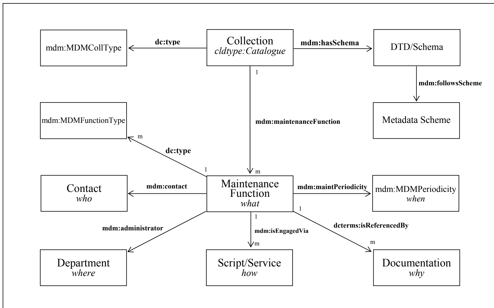
Figure 3. Detailed representation of the properties and resources comprising a metadata maintenance collection description
