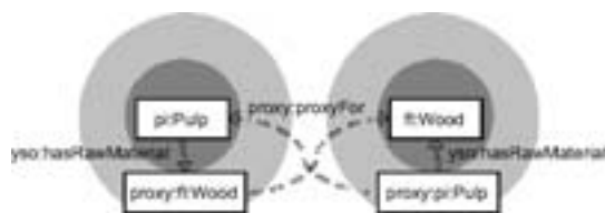
Figure 3: Simple ontologies with proxies providing isolation
