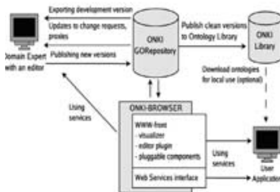
Figure 1: ONKI development and publishing process
