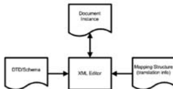
Fig. 4: XML Editor for Multilingual Markup.
