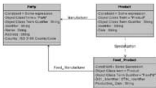
Figure 5. Food datamodel
