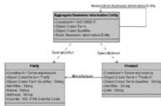
Figure 4. Standard model
