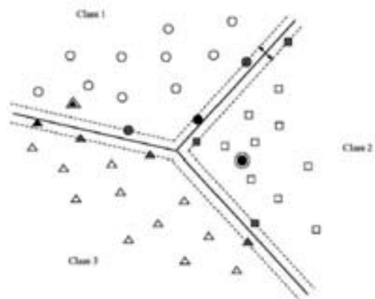
Fig. 3 Multiclass classification problem solved by MSVM. Solid lines represent separating hyperplanes, while dotted lines are hyperplanes which underline the confidence margin. The multiclass margin is the minimal distance between two dotted lines. Dark points are support vectors. Black points are also constraints violations and extra borders indicate violations which are also training errors.
