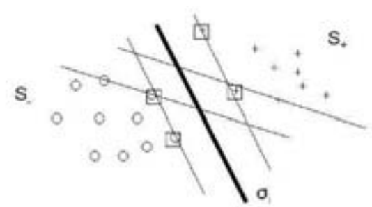
Fig. 2 Geometrical interpretation of the Support Vector Machine method for binary classification of linearly separable examples ( S^+ ( S^- ) are the set of positive (negative) examples; \bullet is the decision surface, boxes indicates the support vectors).
