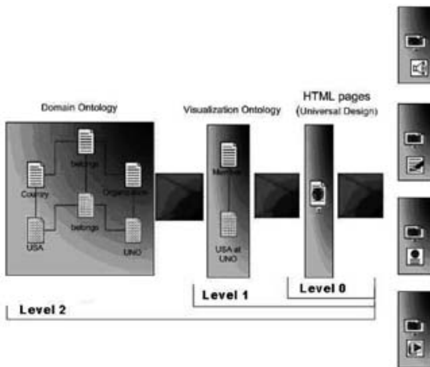
Figure 3: Accessibility through visualization rules in three levels
