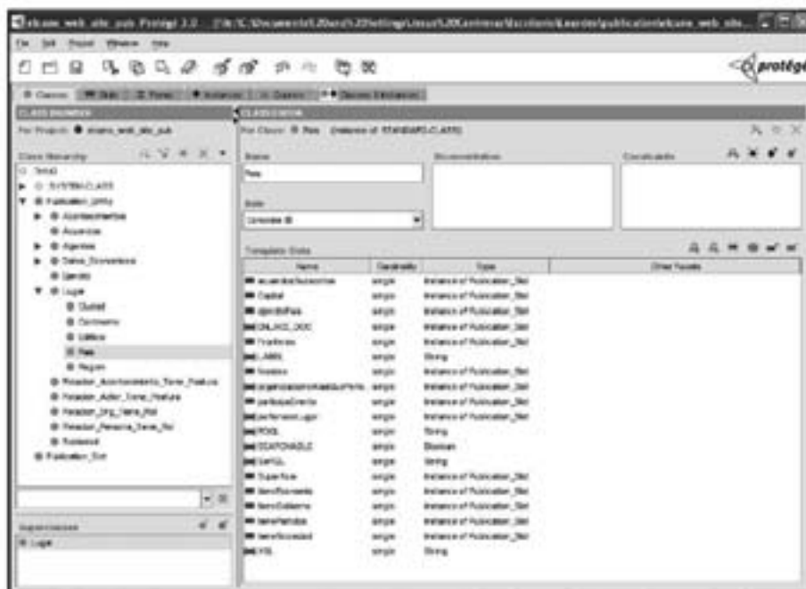
Figure 5: Visualization ontology definition using Protégé.
