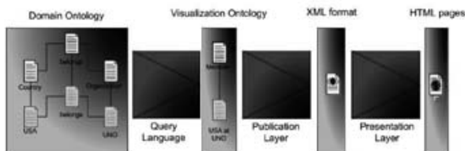
Figure 2: Visualization Ontology Conceptual Model
