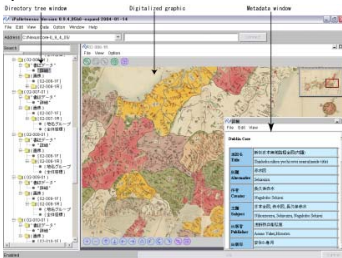
Figure 1. iPalletnexus Interface
