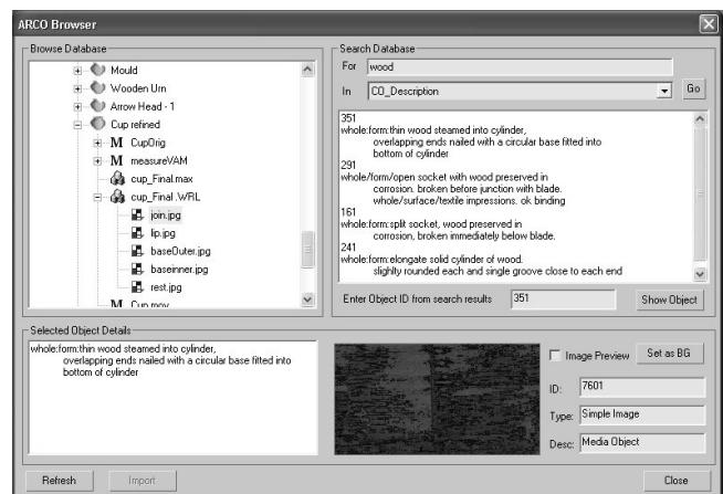
Figure 8. Database plug-in metadata editor
