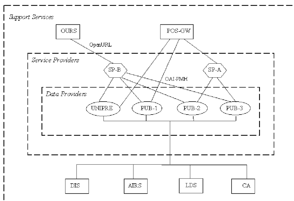
Figure 1. Three-level architecture and a possible deployment scenary
