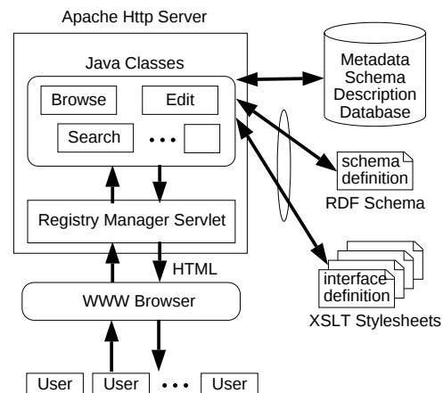
Figure 9. Registry Architecture
