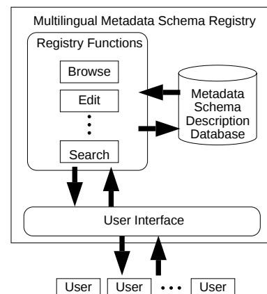
Figure 3. System Architecture of the Metadata Schema Registry
