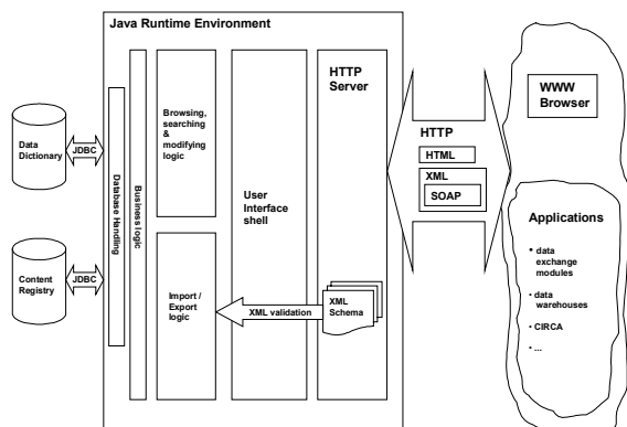
Figure 6: System Architecture
